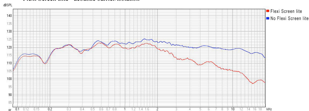
Flexi Screen Lite - acoustic barrier/isolation
