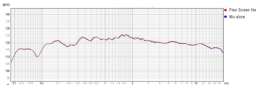
Flexi Screen Lite - microphone response
